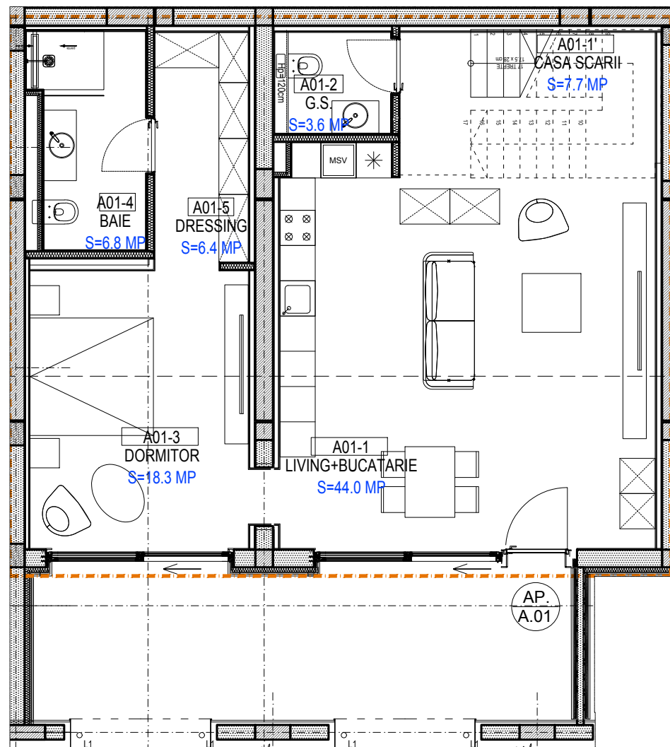
PARTER DUPLEX
