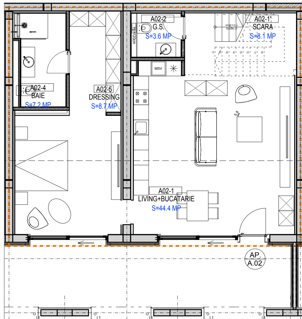
PARTER DUPLEX
